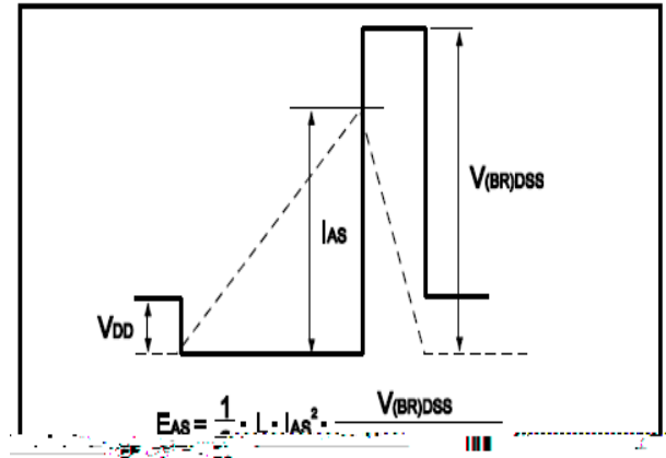
Fig.16 Avalanche Waveform
