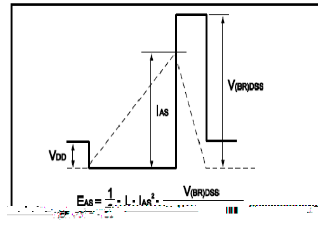
Fig.16 Avalanche Waveform
